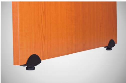
Rectification is intended to compensate for the undulation of floors by up to 1.5 cm
